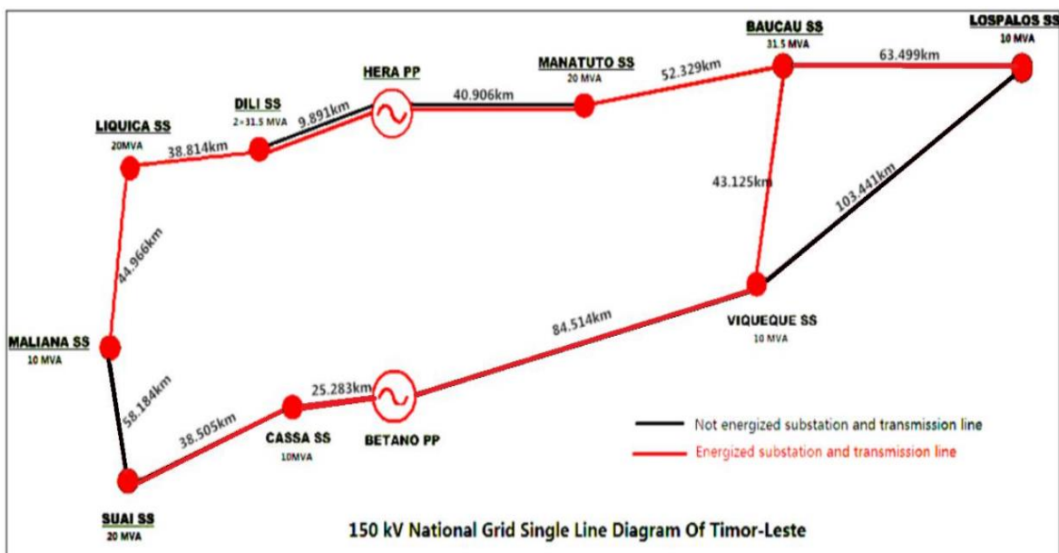
Figura 13 Single Line Diagram 150kV Timor-Leste
